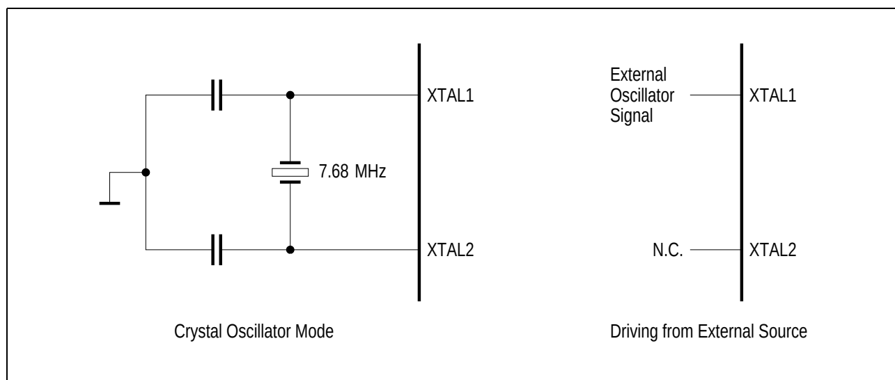
Figure 82 Oscillator Circuits
