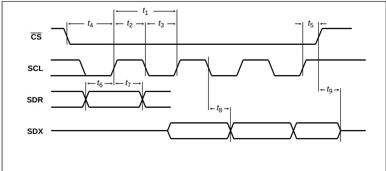
Figure 87 SCI Interface
