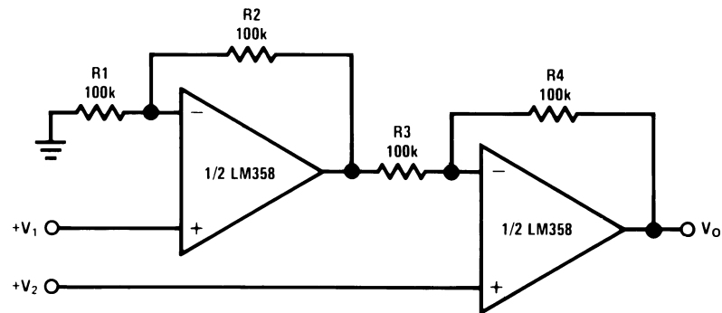
High Input Z, DC Differential Amplifier
