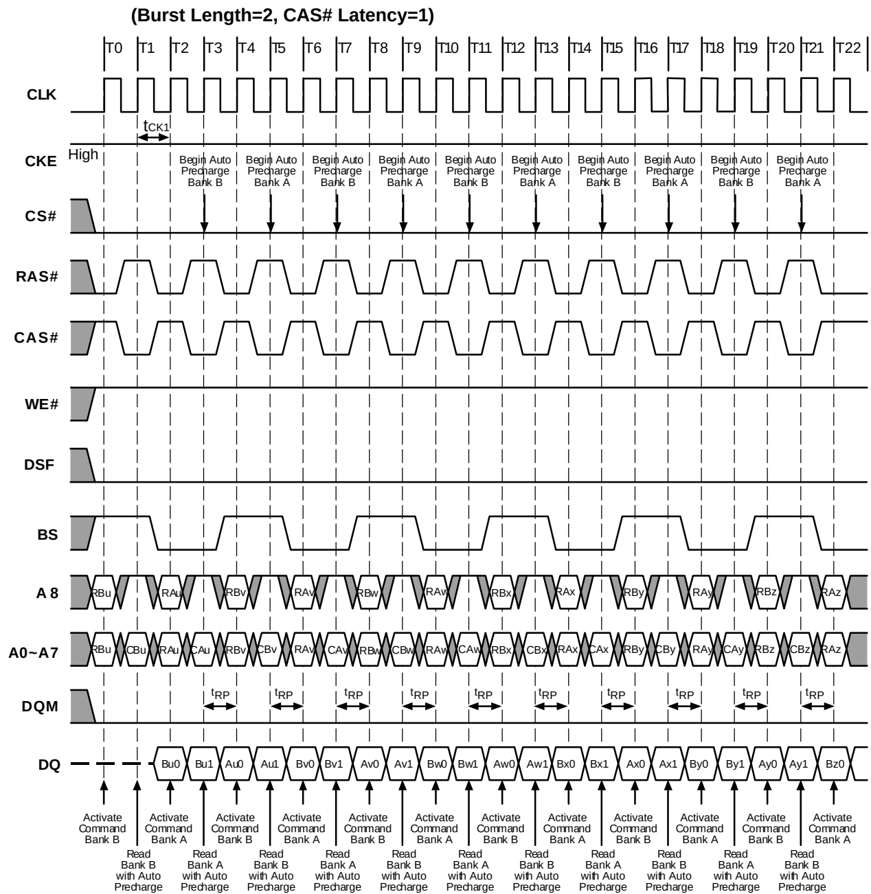
Figure 23. Random Row Read (Interleaving Banks)
