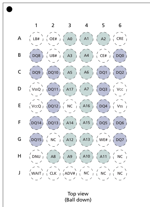
Figure 1: 54-Ball VFBGA Ball Assignment
