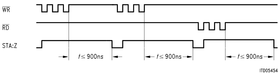
Figure 17 Timing Diagrams of IAR
