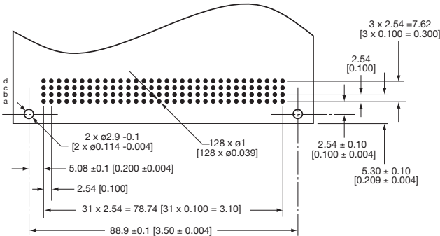
HOLE PATTERN
