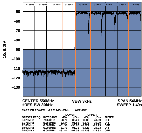
Figure 70. Mid Band Narrow-Band ACLR (Worse Side)
