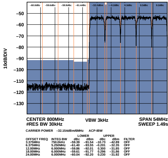
Figure 71. High Band Narrow-Band ACLR
