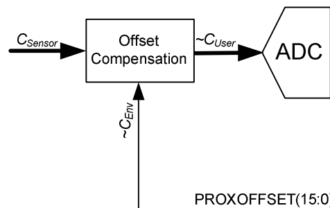
Figure 32 – Offset Compensation Block Diagram
