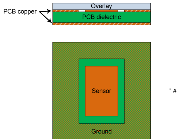
Figure 29 – Typical Capacitive Sensing Implementation
