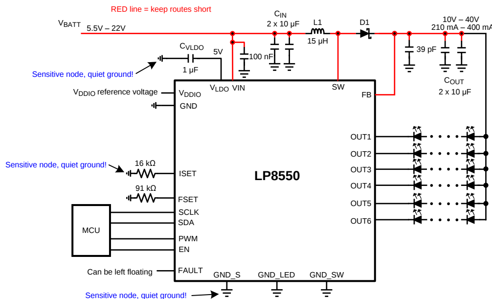
Figure 32. LP8550 Application Schematic for Layout
