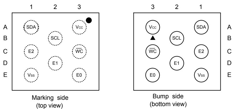
Figure 3. WLCSP connections
