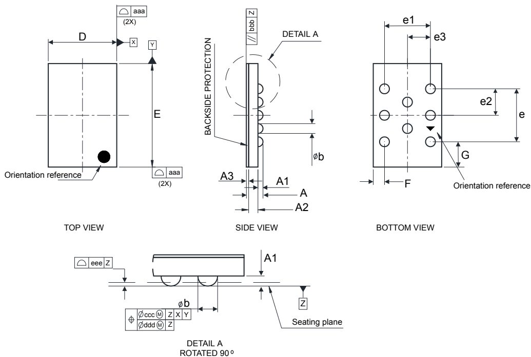
Figure 23. WLCSP8 - Outline
