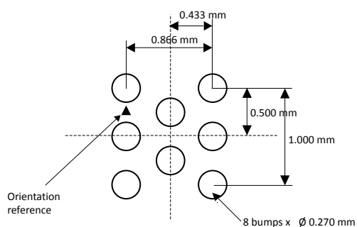
Figure 22. WLCSP8 - Recommended footprint
