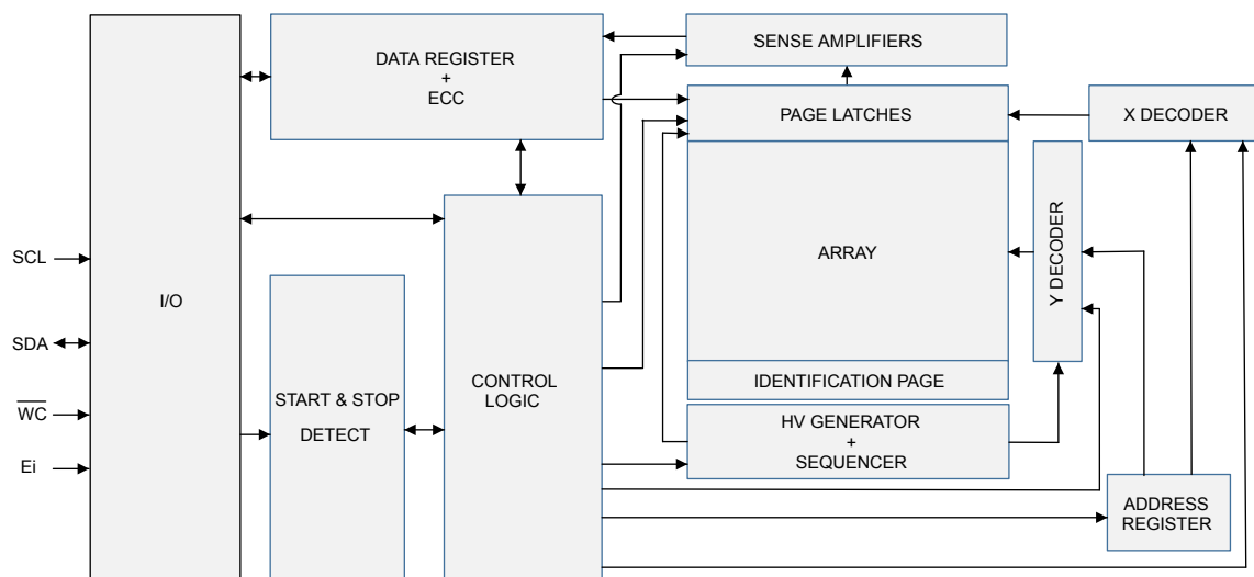
Figure 5. Block diagram
