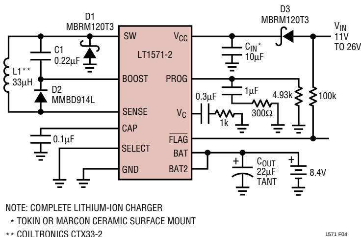
Figure 4. 200kHz Charging Lithium Batteries (Efficiency at 1A > 87%)
