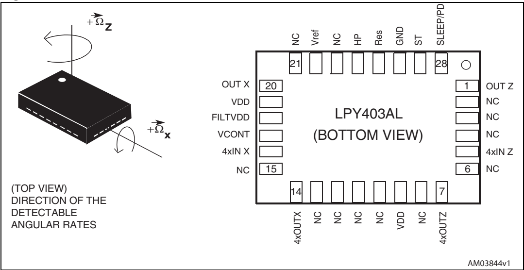
Figure 2. Pin connection
