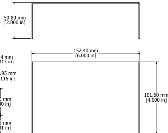
BOTTOM/TOP ENCLOSURE
