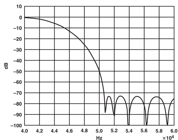
TPC 6. Transition Band Response, 4× Mode
