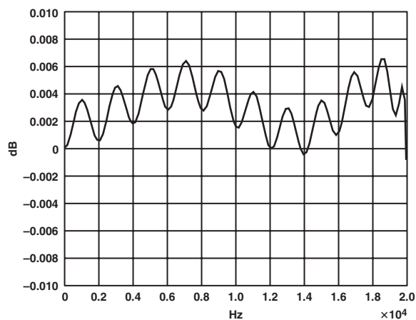
TPC 1. Pass-Band Response, 8× Mode
