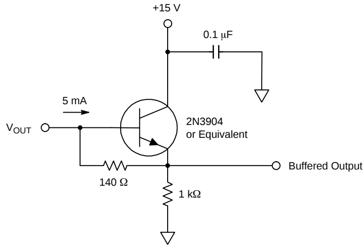
Figure 12. Recommended Output Structure Load Diagram
