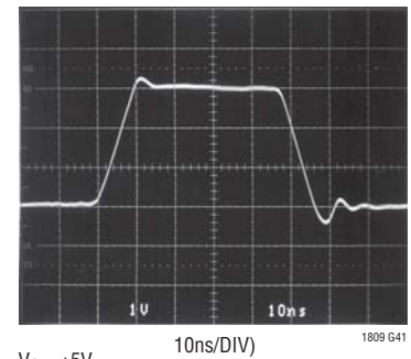
5V Large-Signal Response
