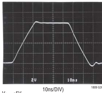
±5V Large-Signal Response
