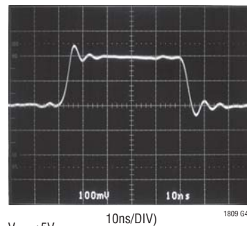
5V Small-Signal Response
