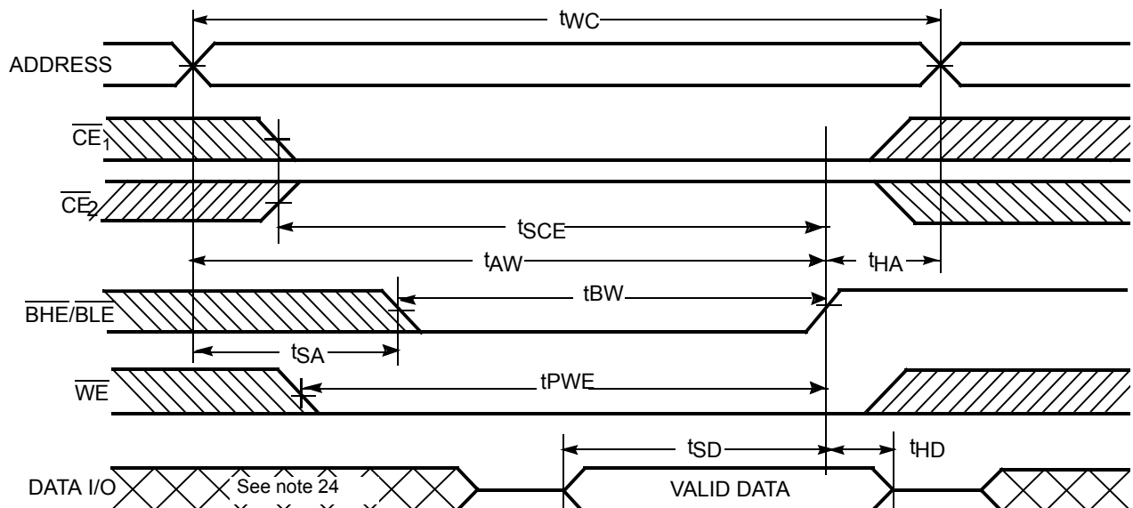
Write Cycle 4 ( \overline{\text{BHE/BLER}} Controlled, \overline{\text{OE}} LOW) [24, 25]
