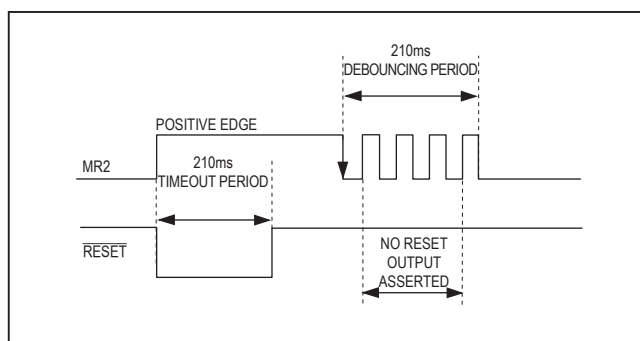
Figure 4. MAX6447/MAX6448/MAX6451/MAX6452 MR2 Deassertion Debouncing Timing Diagram
