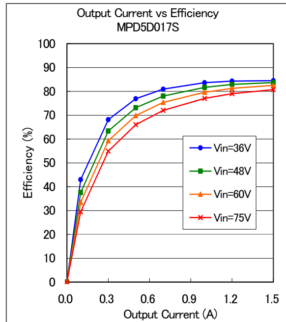
Fig.10.4.2 Efficiency vs Output Current
