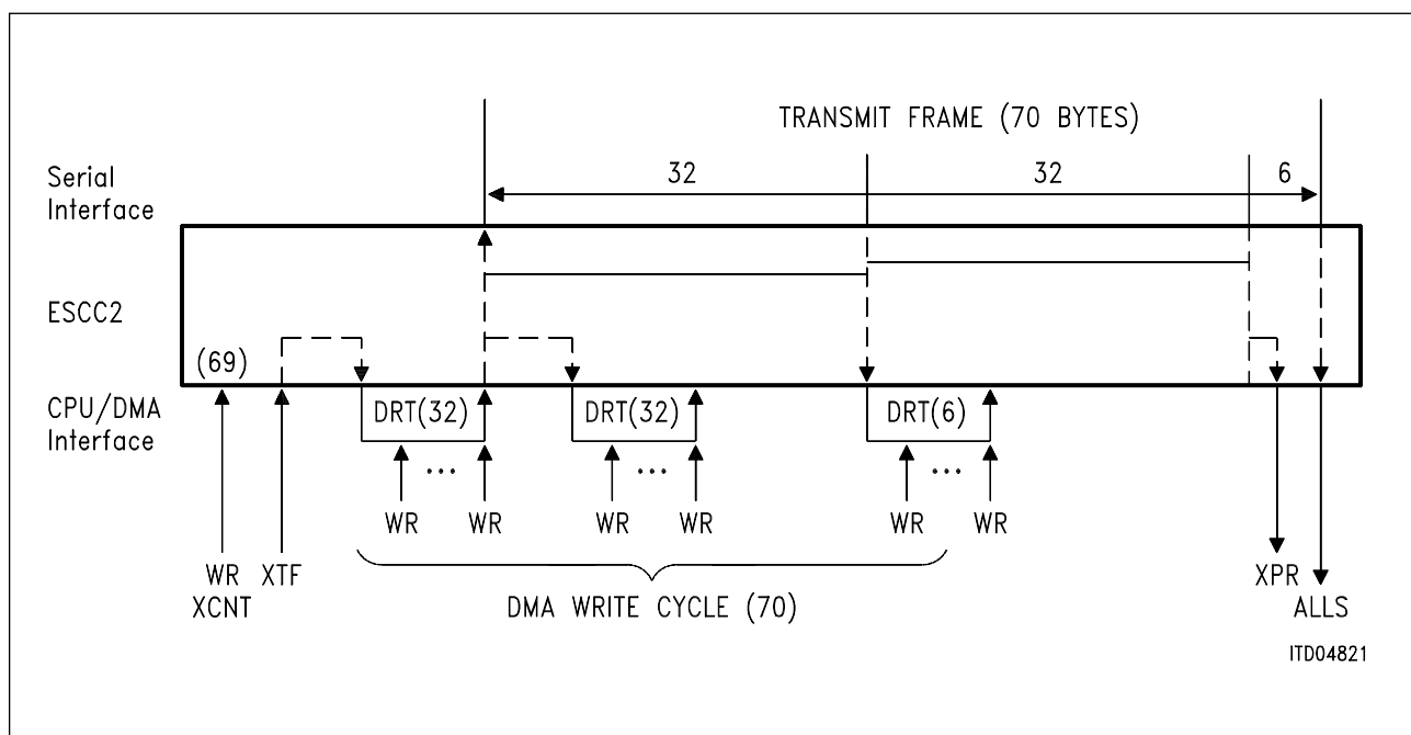
Figure 48 DMA Driven Transmission Sequence Example (HDLC)
