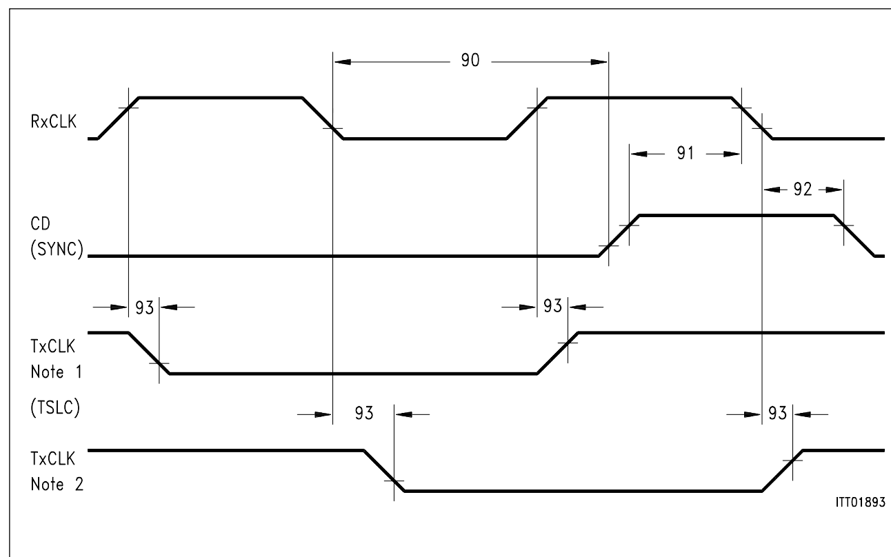
Figure 70 Synchronization Timing
