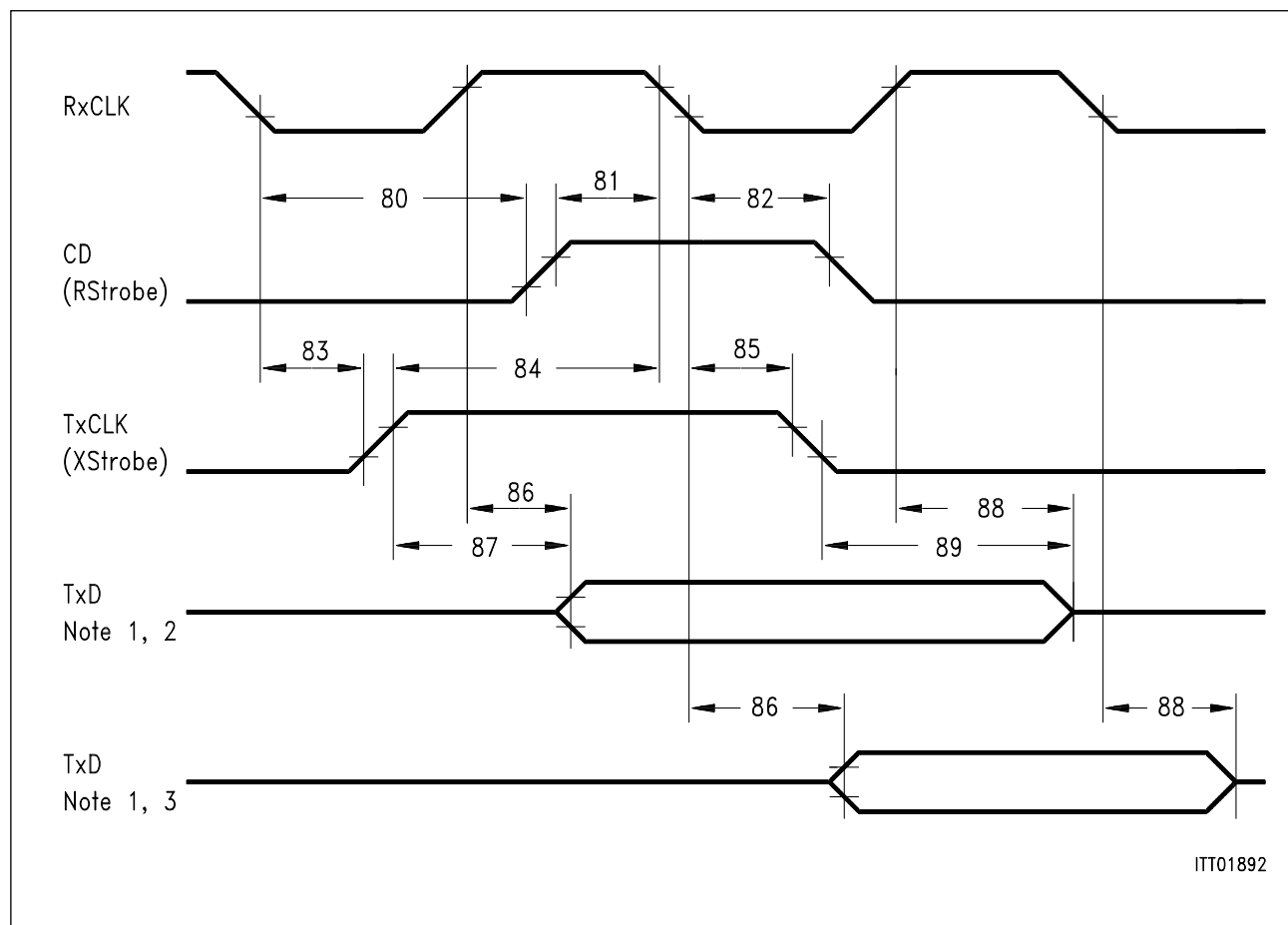
Figure 69 Strobe Timing
