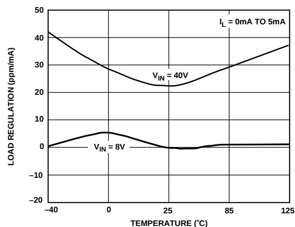
Figure 13. ADR02 Load Regulation vs. Temperature
