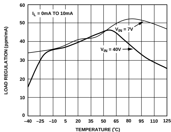
Figure 14. ADR03 Load Regulation vs. Temperature
