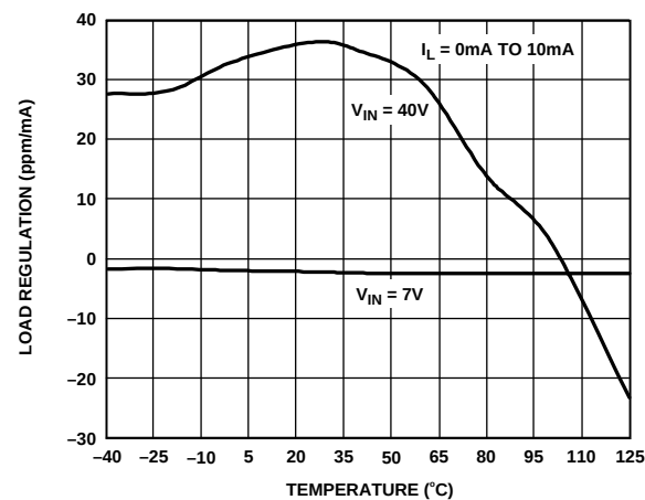
Figure 15. ADR06 Load Regulation vs. Temperature
