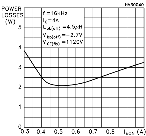
Figure 9. Power losses
