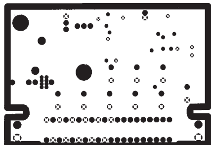
Figure 13. GND Layer
