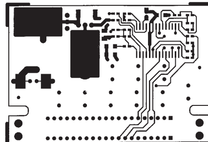
Figure 12. COMP Side
