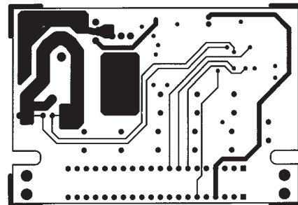
Figure 15. Solder Side
