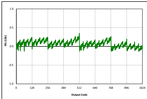
FIGURE 33-80: ADC 10-Bit Mode, Single-Ended INL, V_{DD} = 3.0V , T_{AD} = 4\text{ }\mu s , 25^\circ C .
