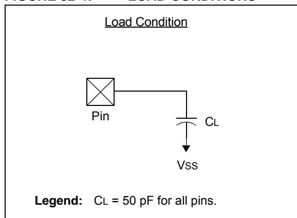
FIGURE 32-4: LOAD CONDITIONS
