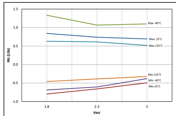
FIGURE 33-84: ADC 10-Bit Mode, Single-Ended INL, V_{DD} = 3.0V , T_{AD} = 1\text{ }\mu s .
