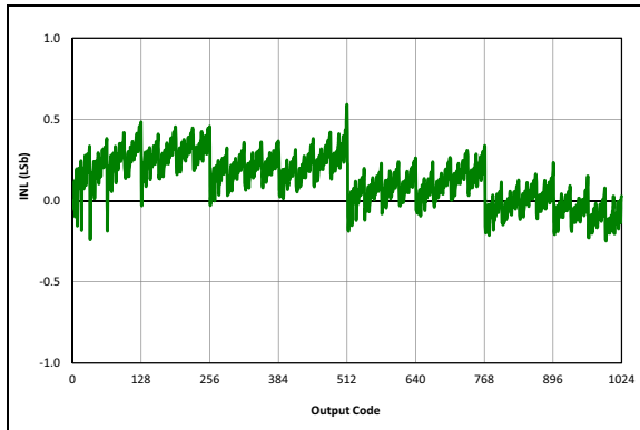
FIGURE 33-79: ADC 10-Bit Mode, Single-Ended INL, V_{DD} = 3.0V , T_{AD} = 1\text{ }\mu s , 25^\circ C .
