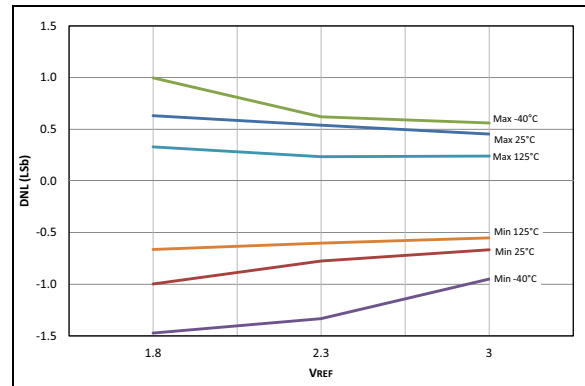
FIGURE 33-83: ADC 10-Bit Mode, Single-Ended DNL, V_{DD} = 3.0V , T_{AD} = 1\text{ }\mu s .
