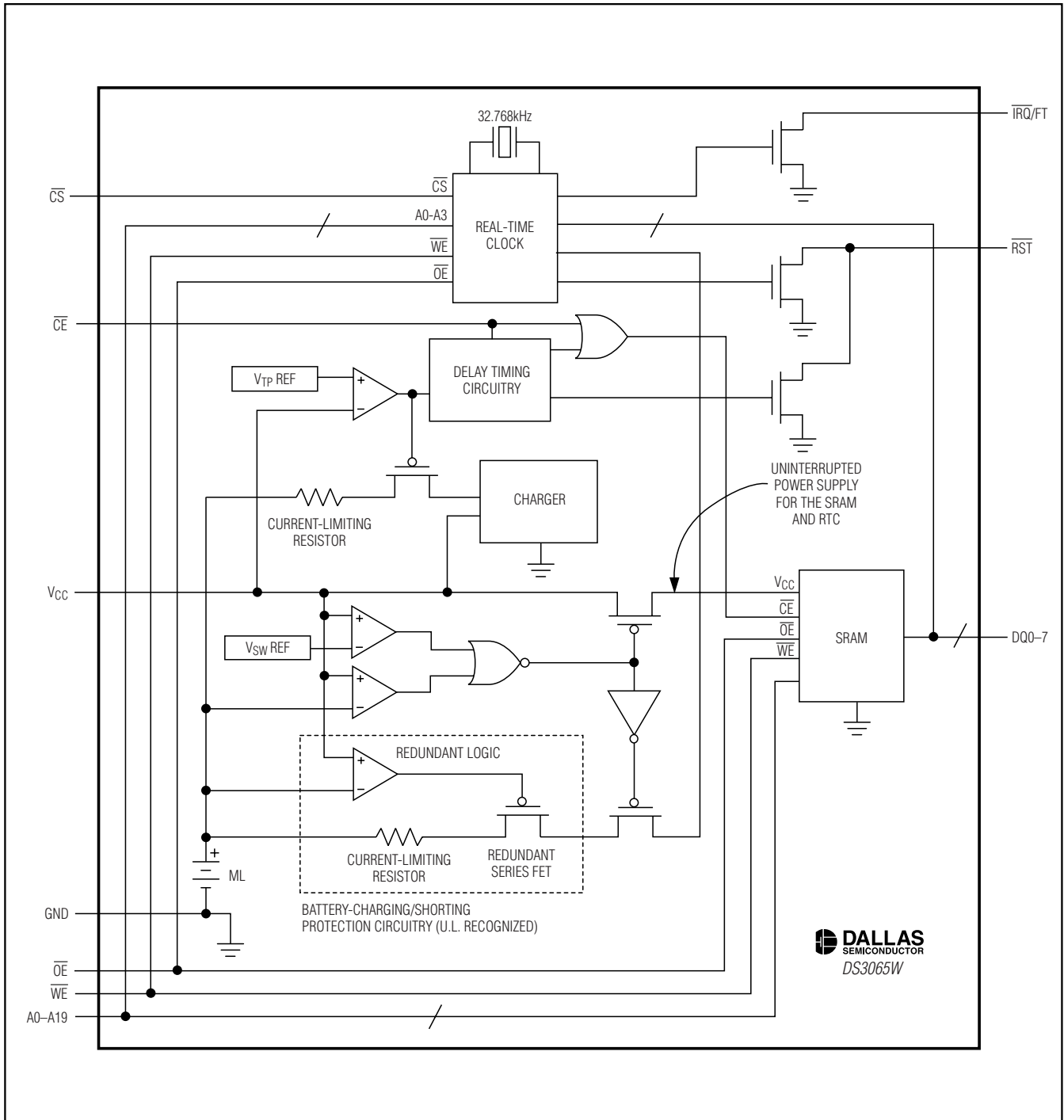
Functional Diagram
