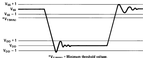
FIGURE 3. Clock Waveform
