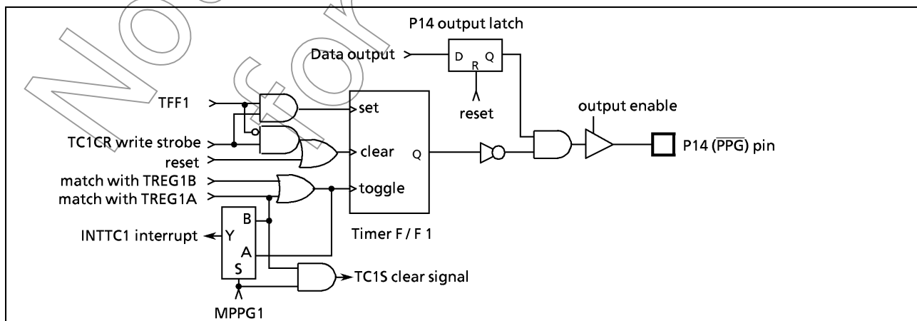
Figure 2-22. PPG Output
