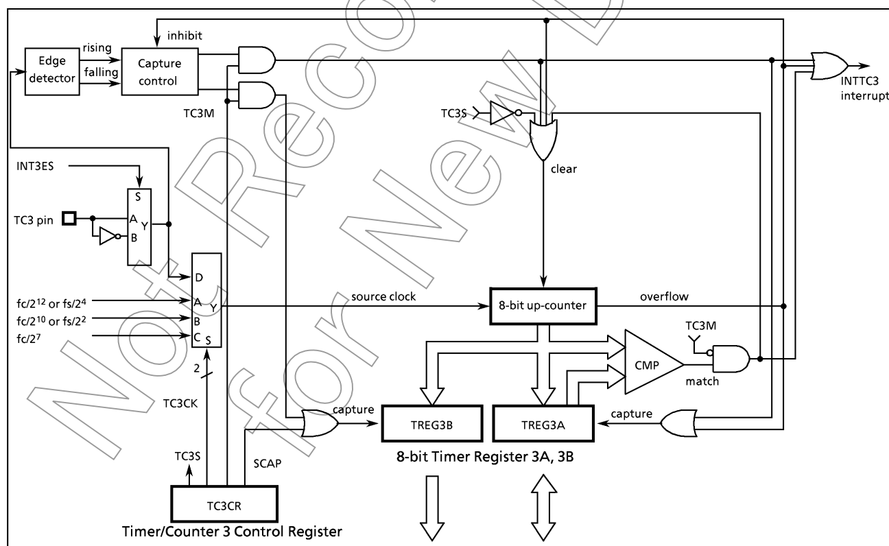
Figure 2-26. Timer/Counter 3
