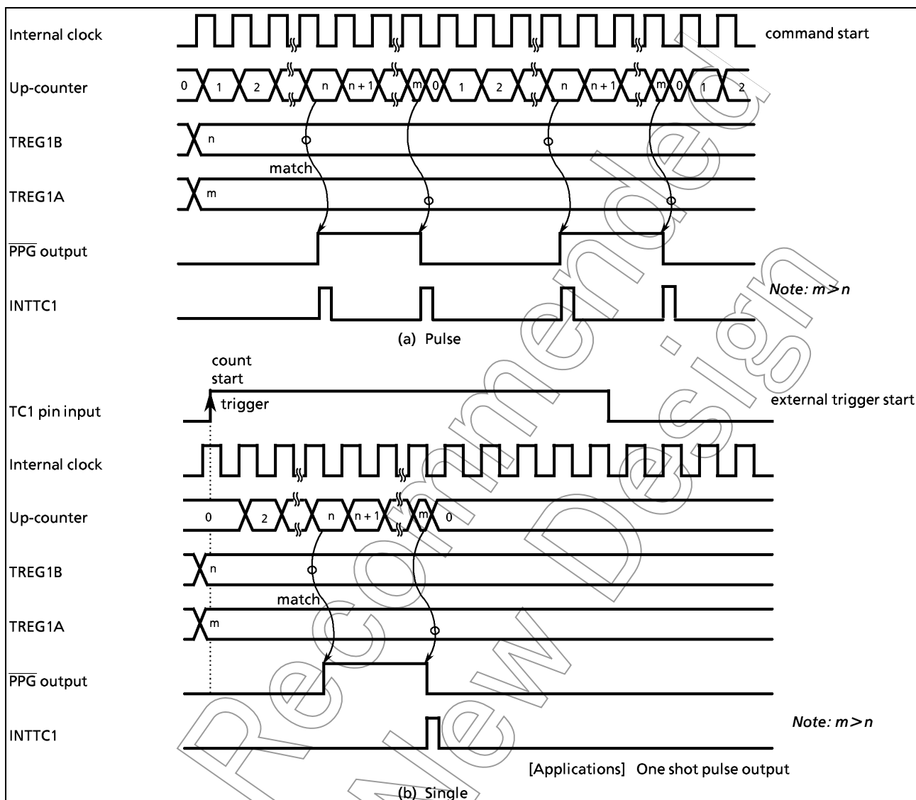
Figure 2-21. PPG Output Mode Timing Chart
