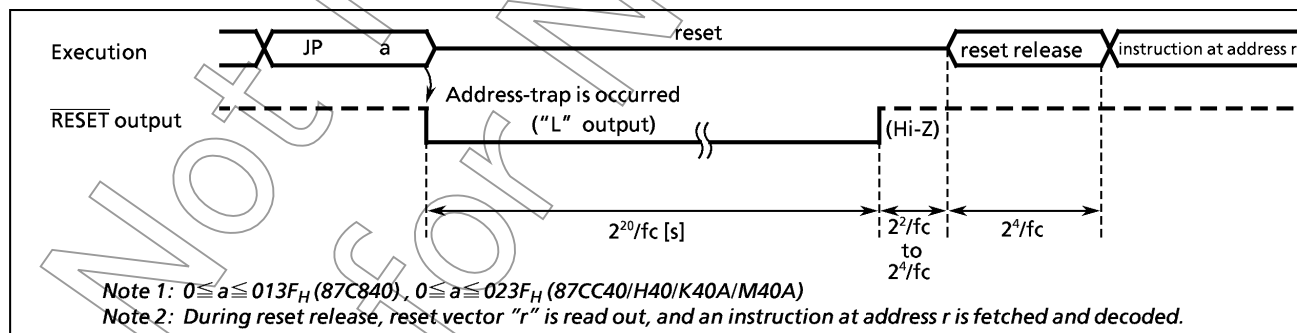
Figure 1-31. Address-Trap-Reset
