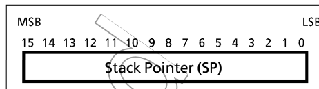
Figure 1-7. Stack Pointer
