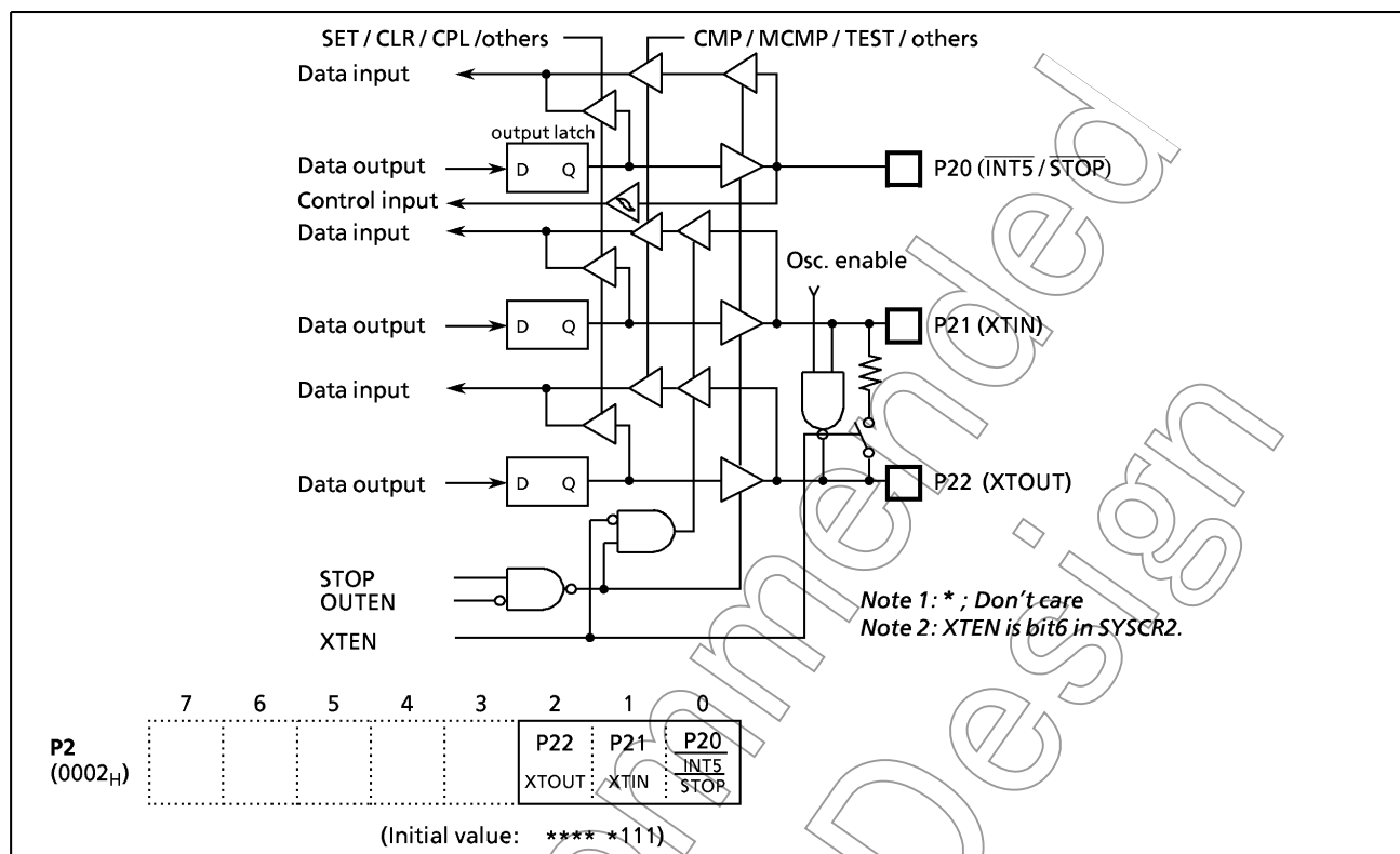
Figure 2-5. Port P2
