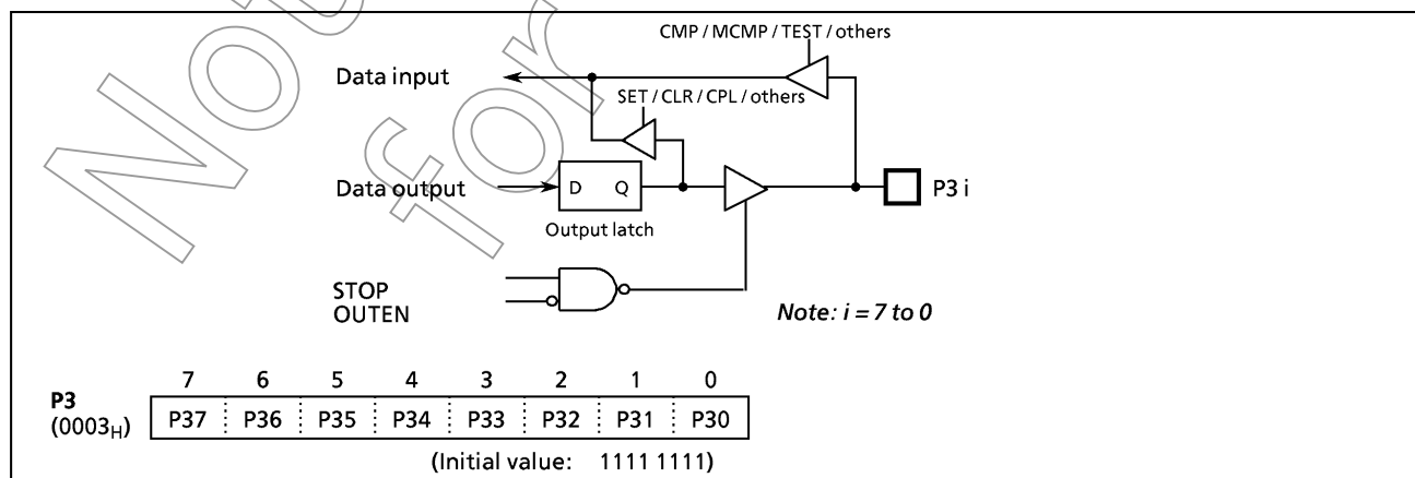
Figure 2-6. Port P3
