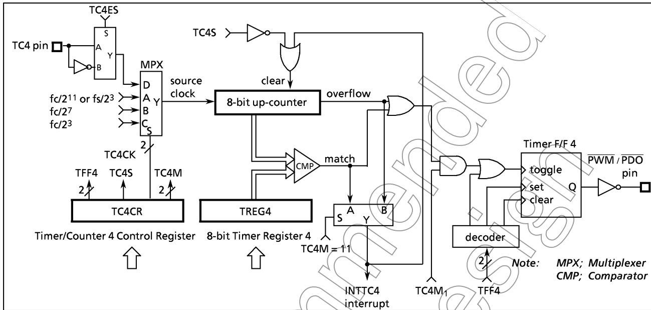
Figure 2-29. Timer/Counter 4
