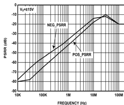
FIGURE 18. POWER SUPPLY REJECTION RATIO (PSRR)
