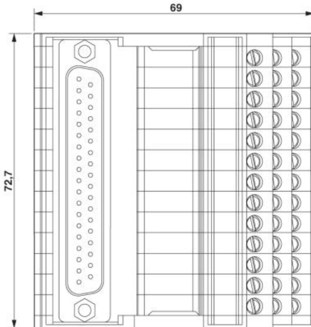
Dimensional drawing
