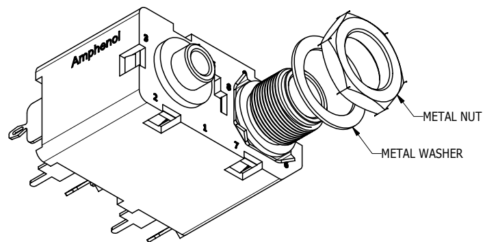
ISO VIEW
