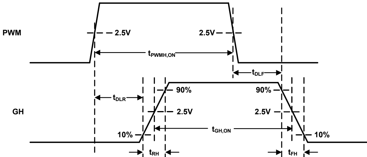
FIGURE 3. TIMING DIAGRAM
