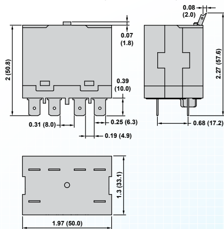
PLUG-IN SOCKET MOUNT (BLADE TERMINAL)
