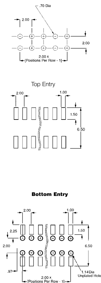
Recommended PCB layouts
