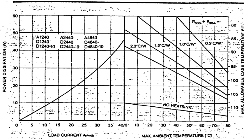
Figure 7. Thermal Derating Curves: 40-Amp, 120/240 and 480V.
