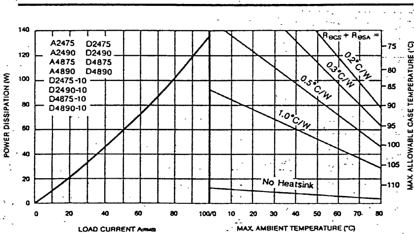
Figure 9. Thermal Derating Curves 75 & 90 Amp, 240 and 480V.
