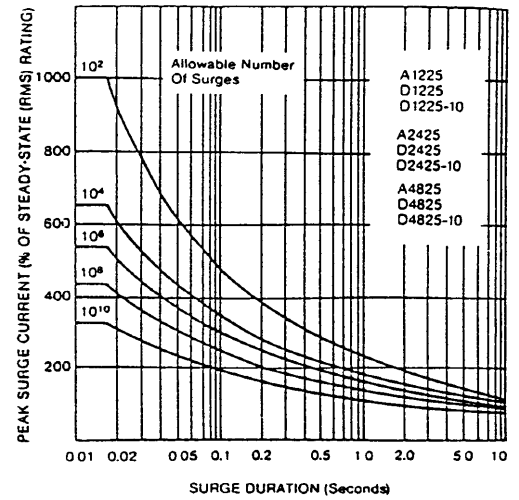
Figure C. Peak Surge Current vs. Duration: 25 Amp Models
