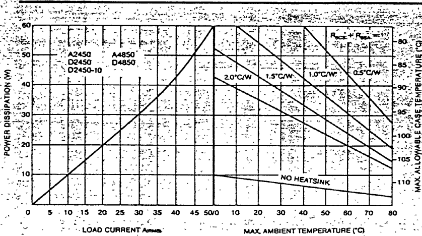
Figure 8. Thermal Derating Curves: 50 Amp, 240V.
