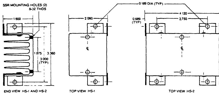
END VIEW HS-1 AND HS-2
