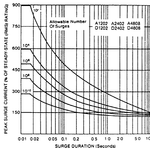
Figure A. Peak Surge Current vs Duration 2 and 8 Amp Models.
