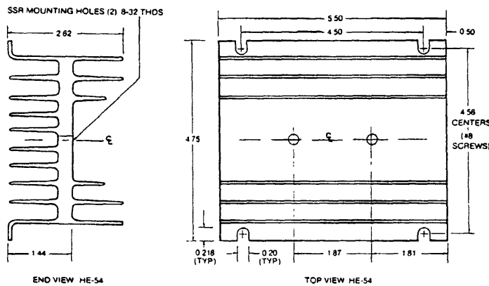
END VIEW HE-54
