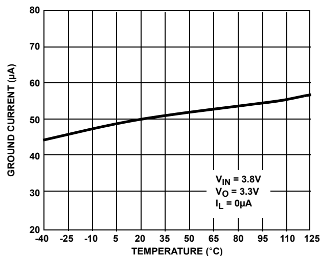
FIGURE 12. GROUND CURRENT vs TEMPERATURE
