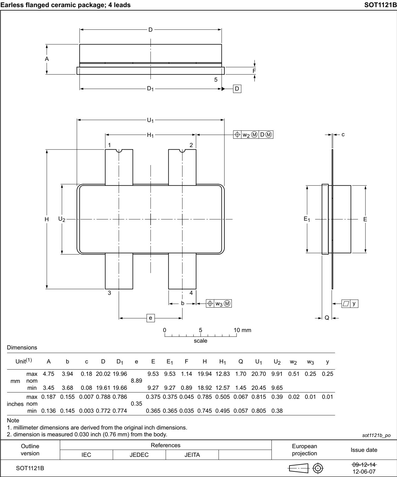
Fig 12. Package outline SOT1121B
