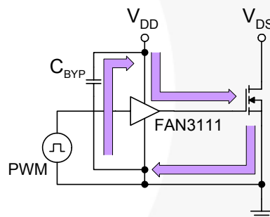
Figure 39. Current Path for MOSFET Turn-On
