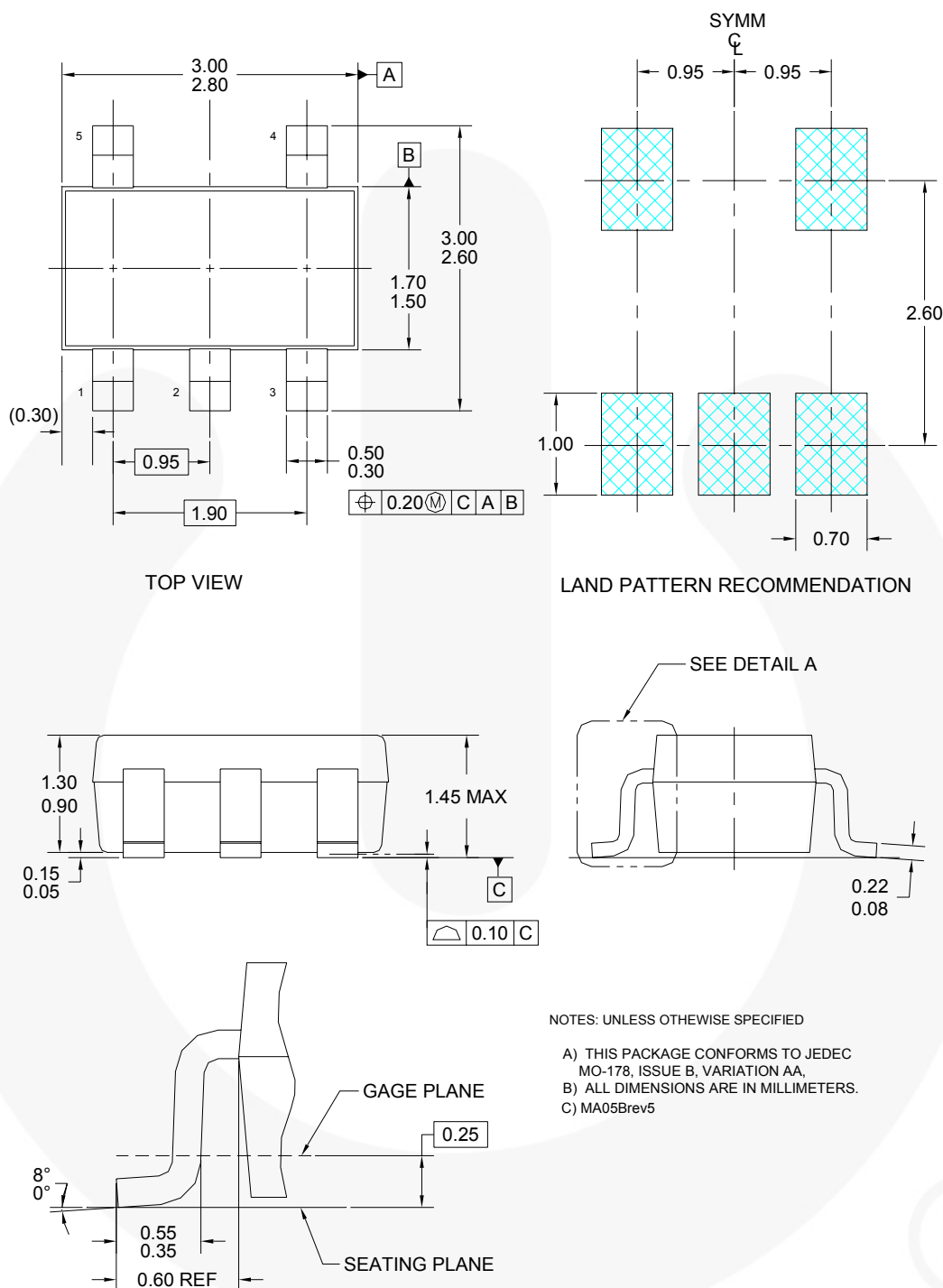
Figure 46. 5-Lead SOT-23
