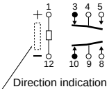
Single side stable (Deenergized condition)
