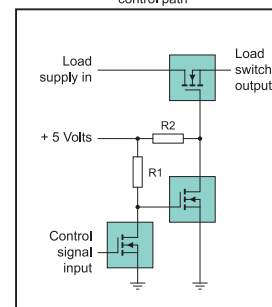
Load Switch with an N-channel FET in the load path and a dual N-channel FET in the control path
