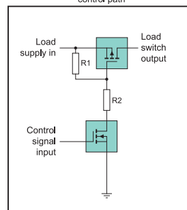
Load Switch with a P-channel FET in the load path and an N-channel FET in the control path
