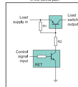
Load Switch with a low V_{CEsat} transistor in the load path and a Resistor-Equipped Transistor in the control path
