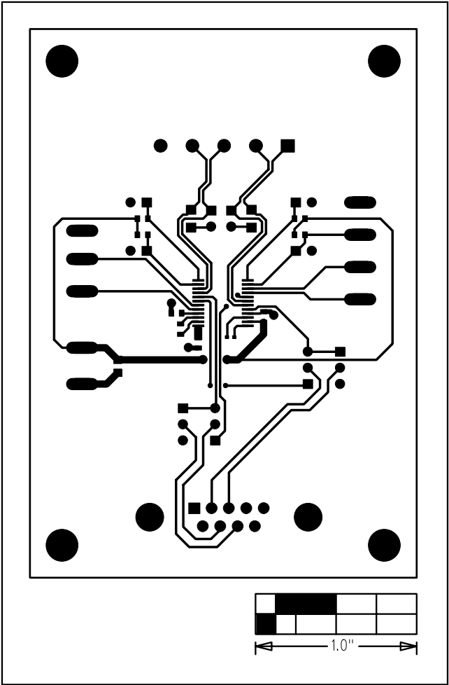
Figure 5. MAX3161E EV Kit PCB Layout—Component Side
