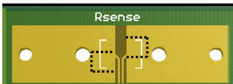
Figure 3: Cutting pads to accommodate 4-wire resistors
