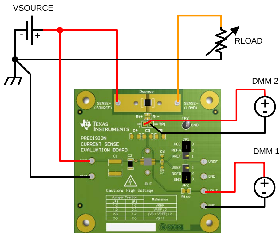
Figure 9: Setup for Bi-Directional Devices
