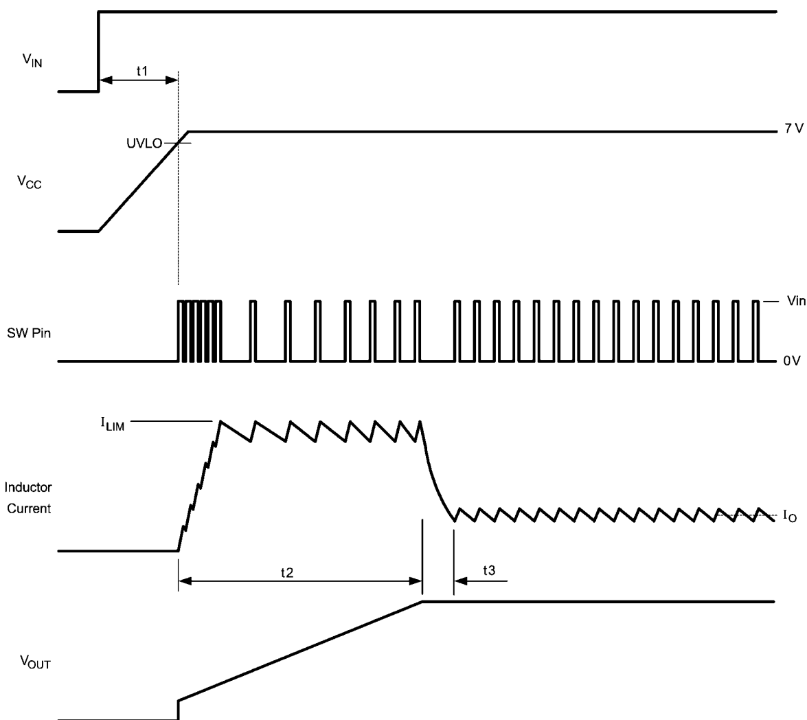
FIGURE 2. Startup Sequence
