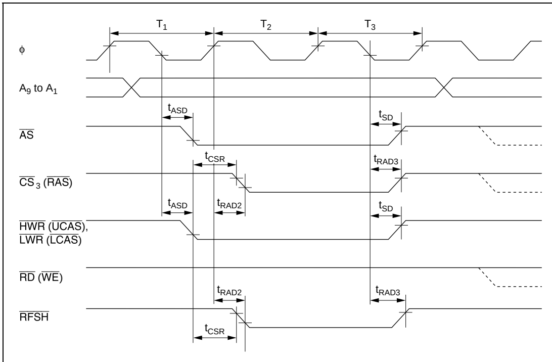
Figure 22.14 DRAM Bus Timing (Refresh Cycle): Three-State Access — \overline{2CAS} Mode —
