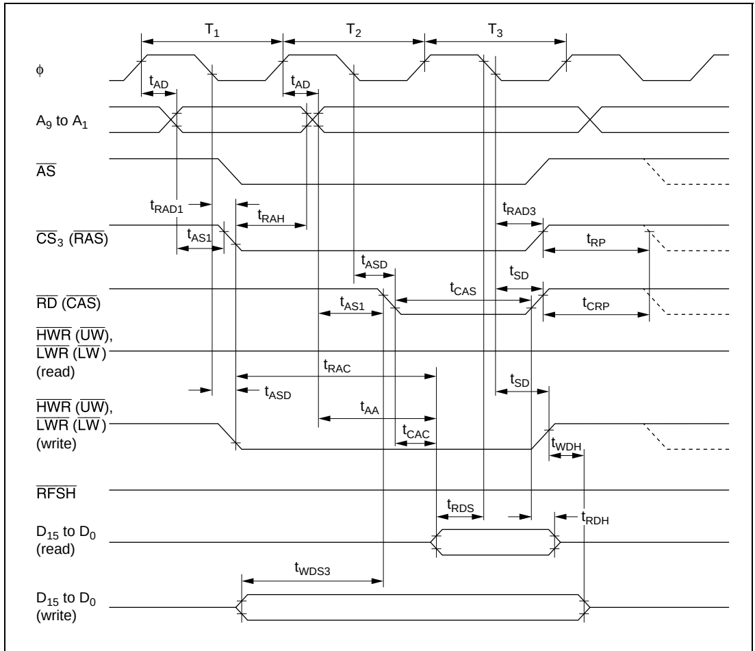
Figure 22.10 DRAM Bus Timing (Read/Write): Three-State Access — 2WE Mode —
