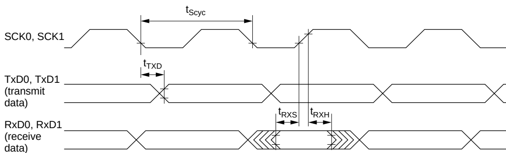
Figure 22.27 SCI Input/Output Timing in Synchronous Mode
