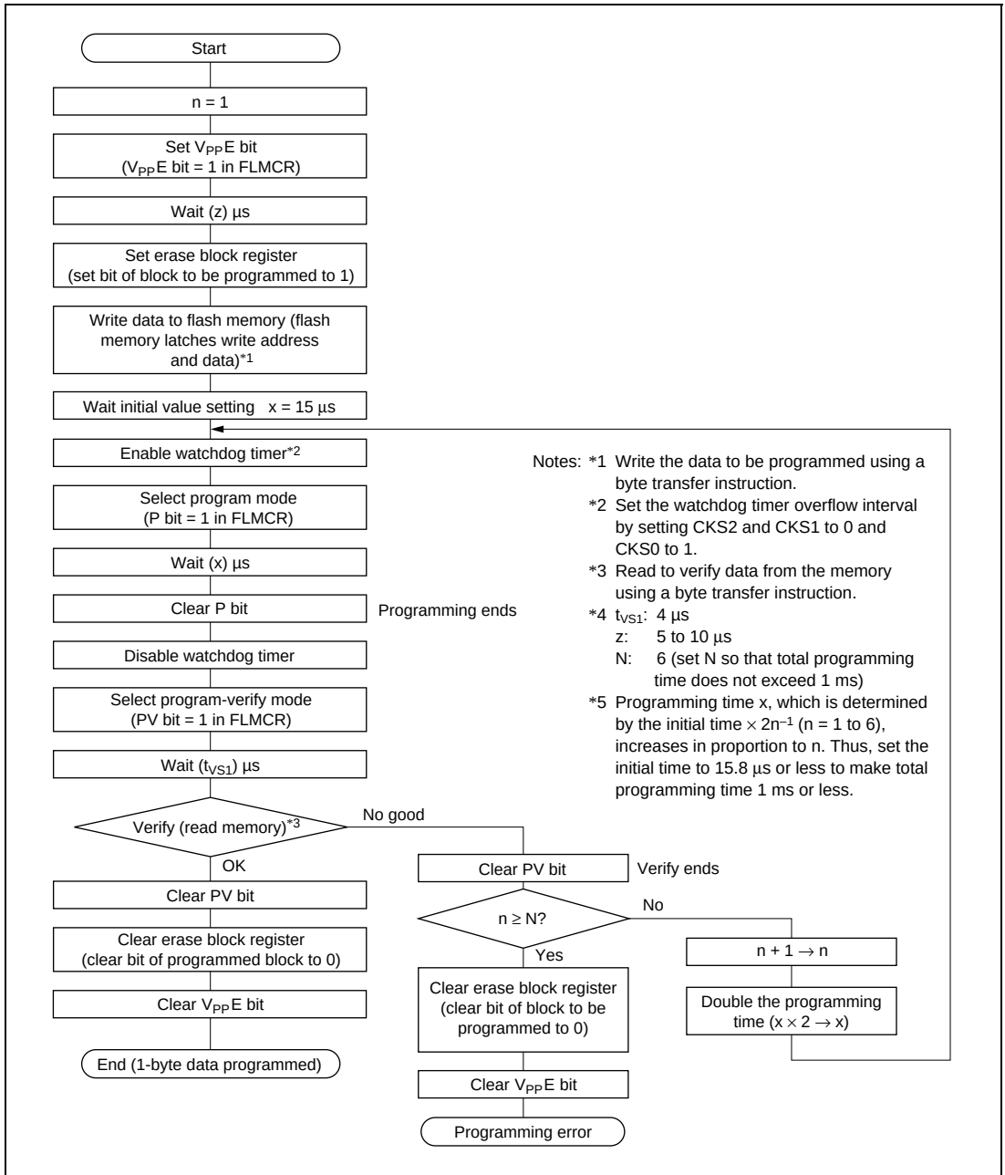
Figure 19.9 Programming Flowchart
