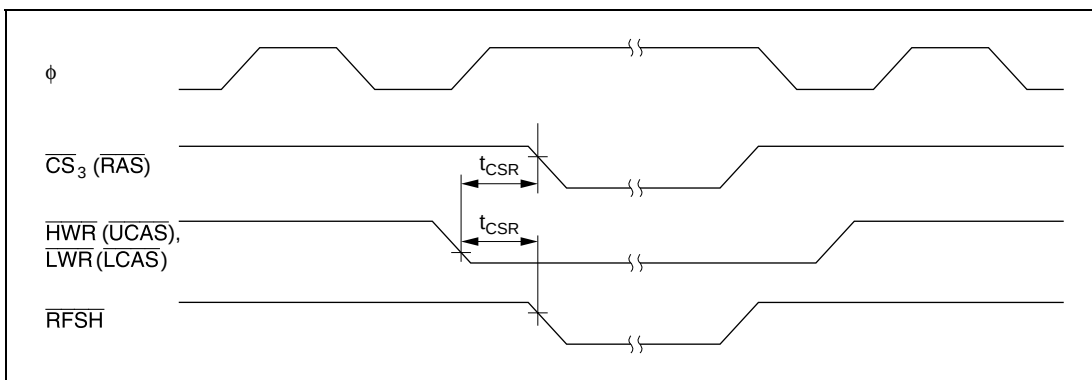
Figure 22.15 DRAM Bus Timing (Self-Refresh Mode) — \overline{2CAS} Mode —
