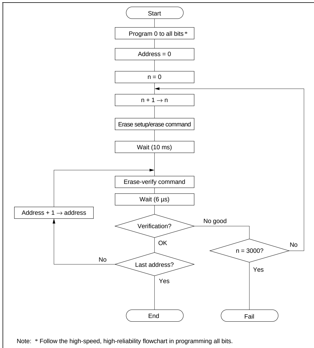
Figure 19.18 High-Speed, High-Reliability Erasing
