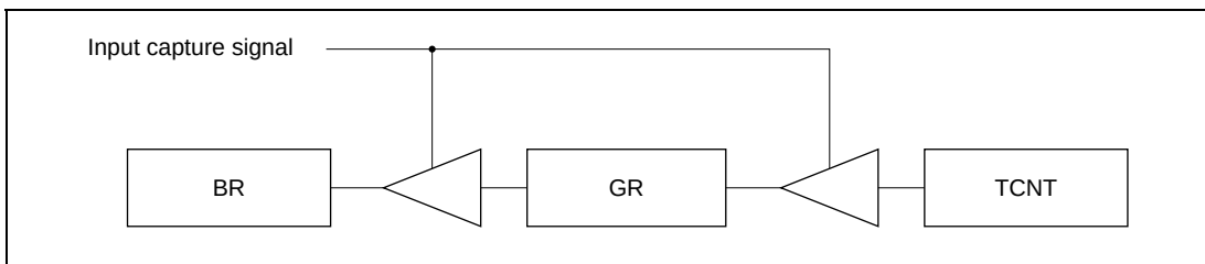
Figure 10.47 Input Capture Buffering
