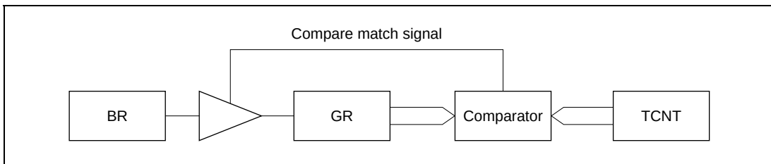
Figure 10.46 Compare Match Buffering
