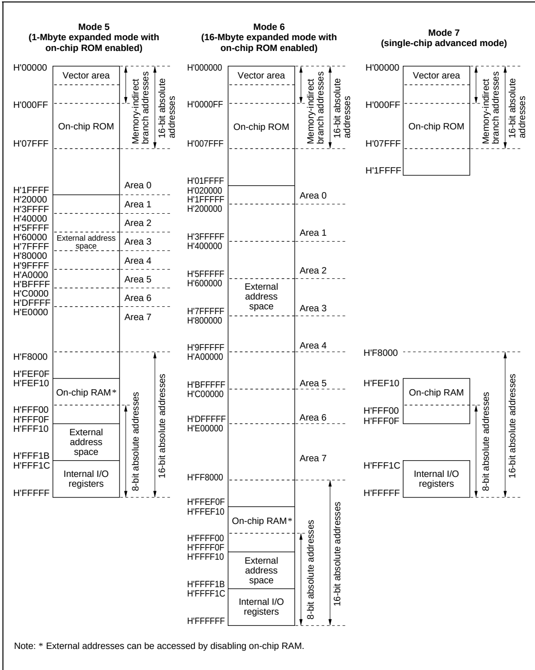
Figure 3.1 H8/3048 Memory Map in Each Operating Mode (cont)
