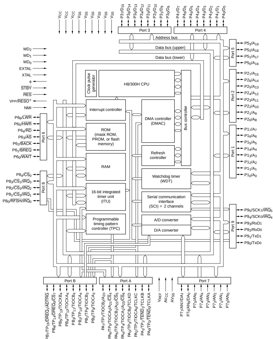
Figure 1.1 Block Diagram
