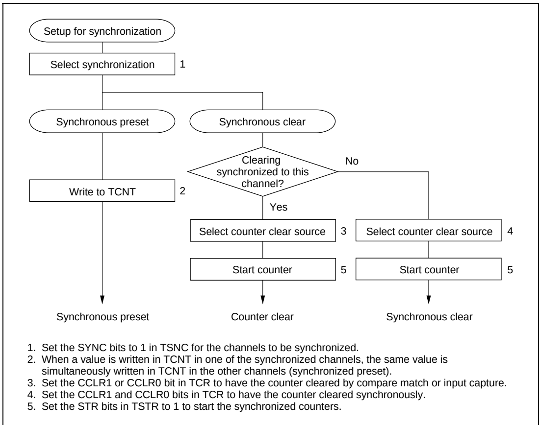
Figure 10.26 Setup Procedure for Synchronization (Example)
