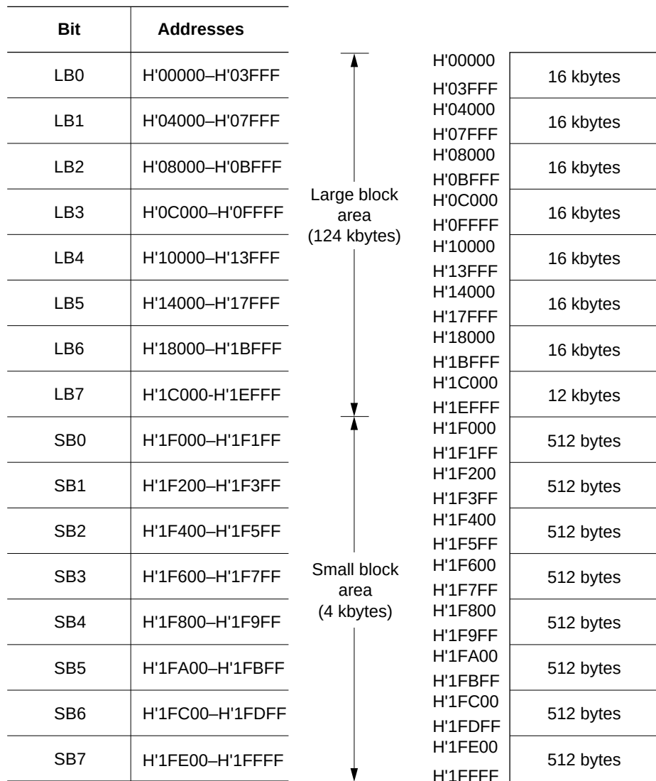
Figure 19.2 Erase Block Map
