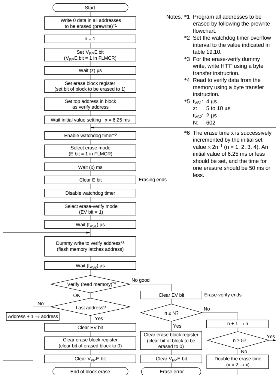
Figure 19.10 Erasing Flowchart
