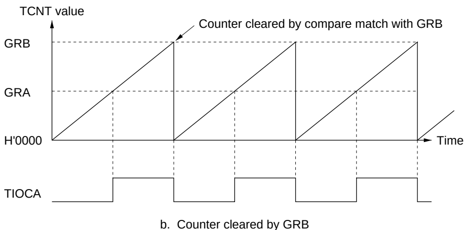
Figure 10.29 PWM Mode (Example 1)
