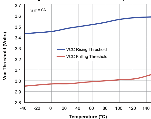
Fig 8. V_{CC} UVLO Threshold vs. Temperature
