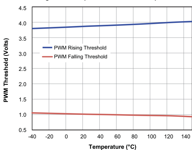
Fig 9. PWM Input Threshold vs. Temperature
