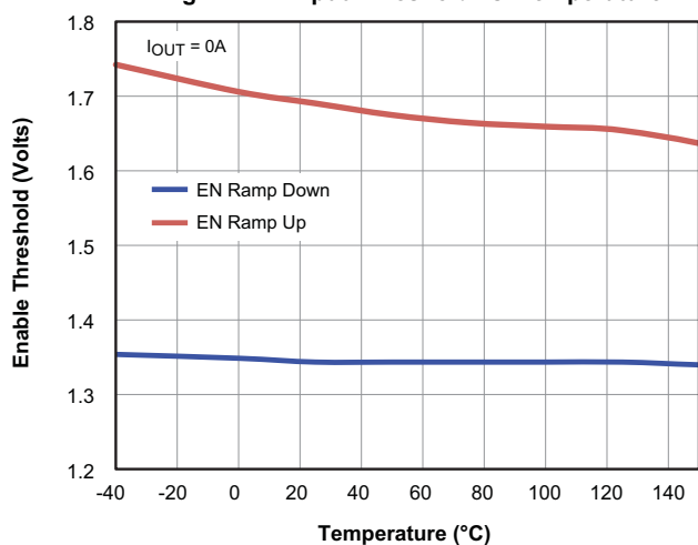
Fig 11. EN Input Threshold vs. Temperature
