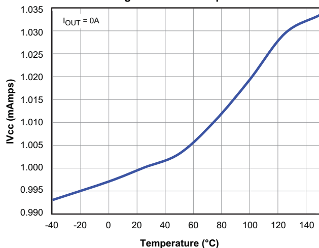
Fig 7. I_{VCC} vs. Temperature
