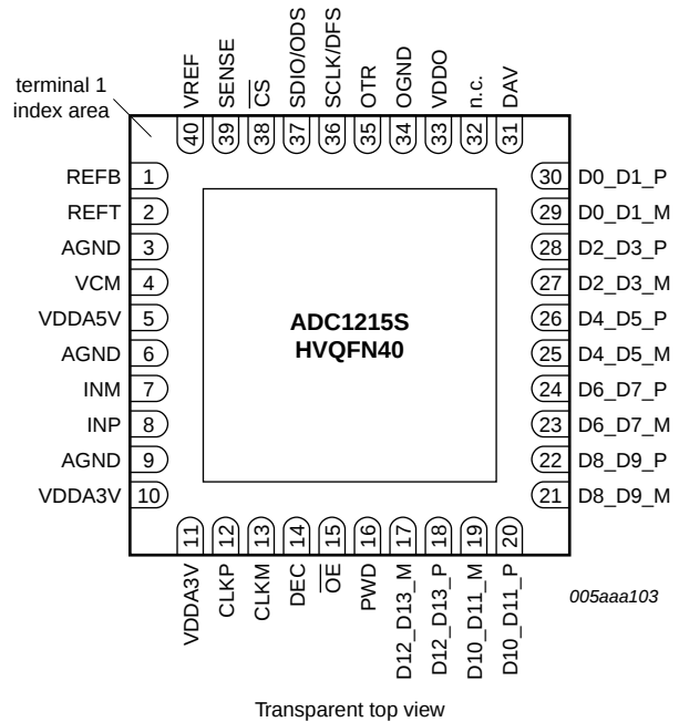
Fig 3. Pin configuration with LVDS/DDR digital outputs selected
