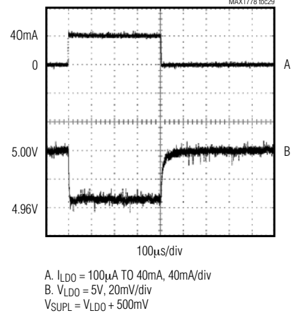
LOAD-TRANSIENT RESPONSE (INTERNAL LINEAR REGULATOR)
