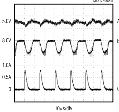
INTERNAL LINEAR-REGULATOR RIPPLE REJECTION
