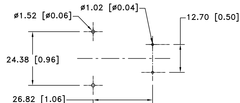
PCB LAYOUT
