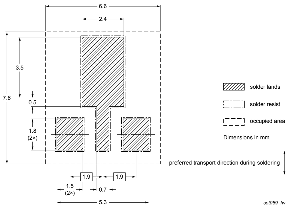
Fig. 14. Wave soldering footprint for SOT89
