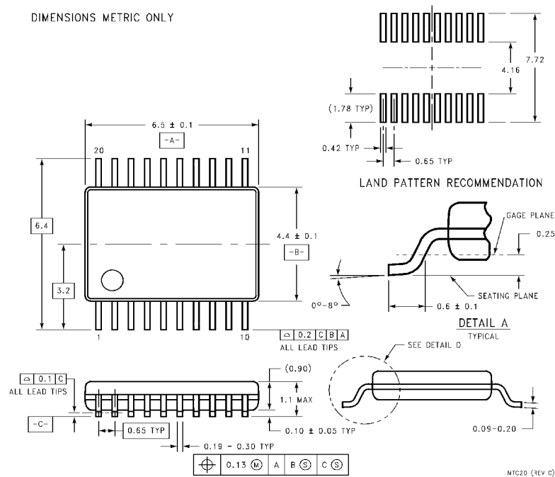
20-Lead Molded Thin Shrink Small Outline Package, JEDEC Package Number MTC20
