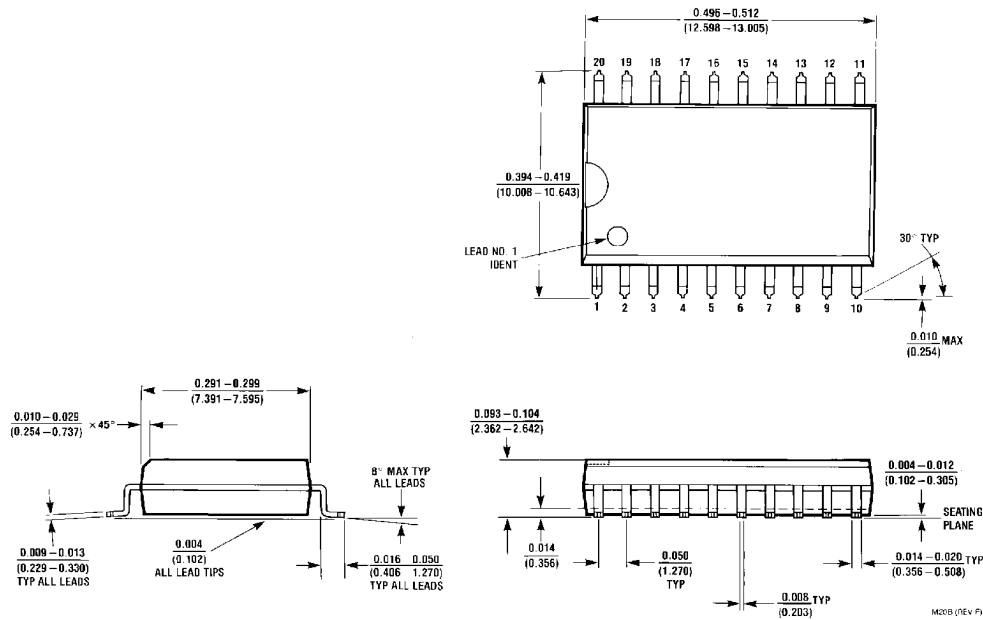
20-Lead Small Outline Integrated Circuit—JEDEC SOIC (M) Package Number M20B
