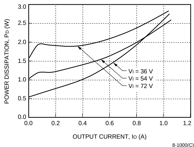
Figure 17. 12 V Output Power Dissipation vs. Output Current
