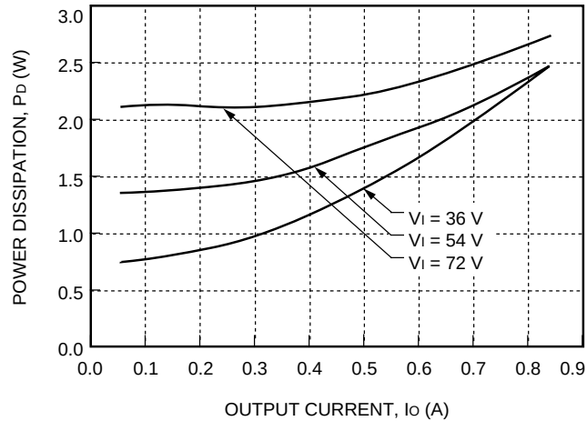
Figure 18. 15 V Output Power Dissipation vs. Output Current
