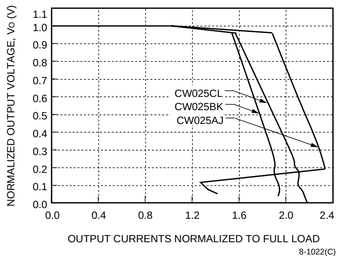
Figure 2. CW025 Dual Output-Series Normalized Output Current vs. Normalized Output Voltage at V_i = 48\text{ V} and T_c = 25^\circ\text{C}
