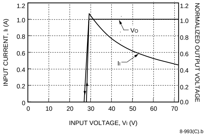
Figure 1. CW025 Dual Output-Series Input Current and Normalized Output Voltage vs. Input Voltage at Full Load and T_c = 25^\circ\text{C}
