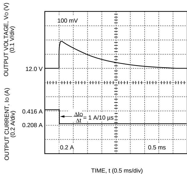
Figure 5. CW025 Dual Output-Series Typical 12 V Output Voltage Response to a Step Load Change from 50% to 25% of I_{o,max} at V_i = V_{i,nom} and T_c = 25^\circ\text{C}
