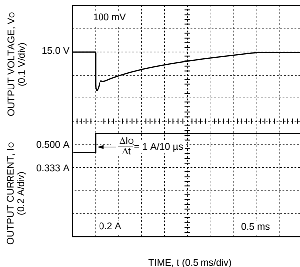
Figure 9. CW025 Dual Output-Series Typical 15 V Output Voltage Response to a Step Load Change from 50% to 75% of I_{o, \max} at V_i = V_{i, \text{nom}} and T_c = 25^\circ\text{C}
