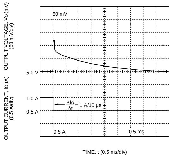
Figure 4. CW025 Dual Output-Series Typical 5 V Output Voltage Response to a Step Load Change from 50% to 25% of I_{o,max} at V_i = V_{i,nom} and T_c = 25^\circ\text{C}
