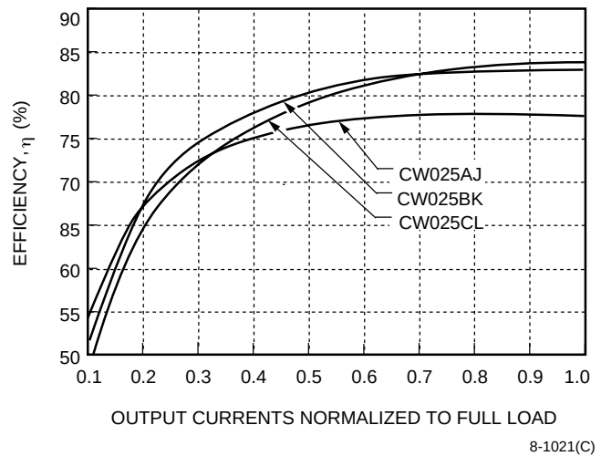
Figure 3. CW025 Dual Output-Series Efficiency vs. Normalized Output Currents (Equal Load on Both Outputs) at V_i = 48\text{ V} and T_c = 25^\circ\text{C}
