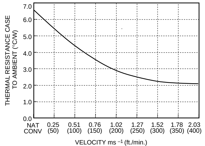
Figure 20. Case-to-Ambient Thermal Resistance vs. Air Velocity
